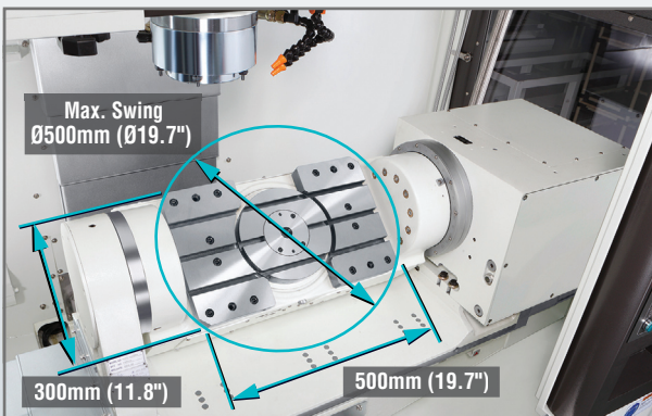
Machine multiple surfaces in one set-up with the Mycenter-3XVT's 5-axis machining capability. Easy and expansive table access streamline and simplify workpiece loading and unloading for larger diameter parts at the same time offering flexibility in fixture set-up for smaller part processing.
